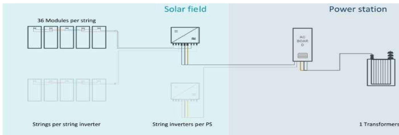
Figure 3. 3: Simplified Electrical Configuration
