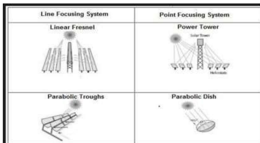
Figure 2. 4: Four different types of solar collector designs (Source: The end of CSP as we know it? | Energiek (wordpress.com) )
