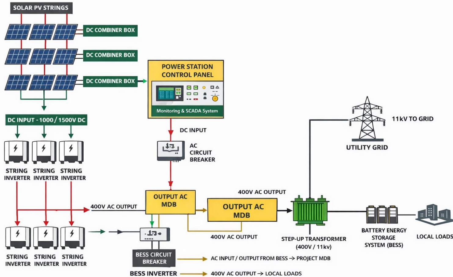
Figure 3. 9: Power station Single line Diagram (Source: EEP3 FEED)
