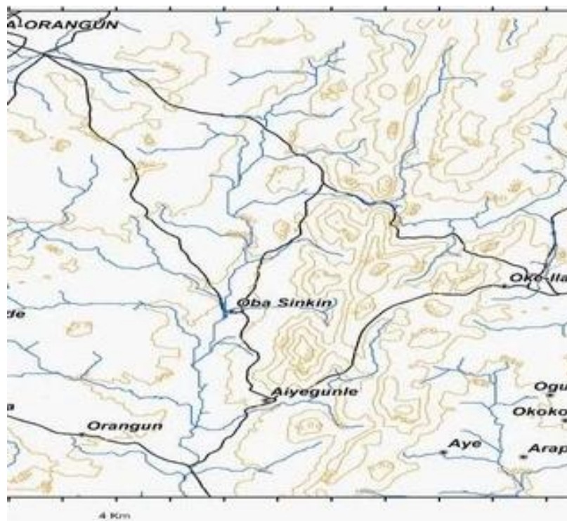
Figure 4.3 Topographic Map of Ila Orangun and Its Environ Source: Afolabi Jayeola et al (2023)
