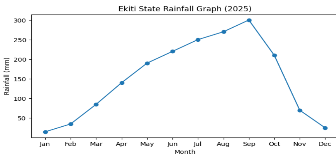
Figure 4.2: Monthly Rainfall in the Proposed Project Area (Source: NIMET, 2025)
