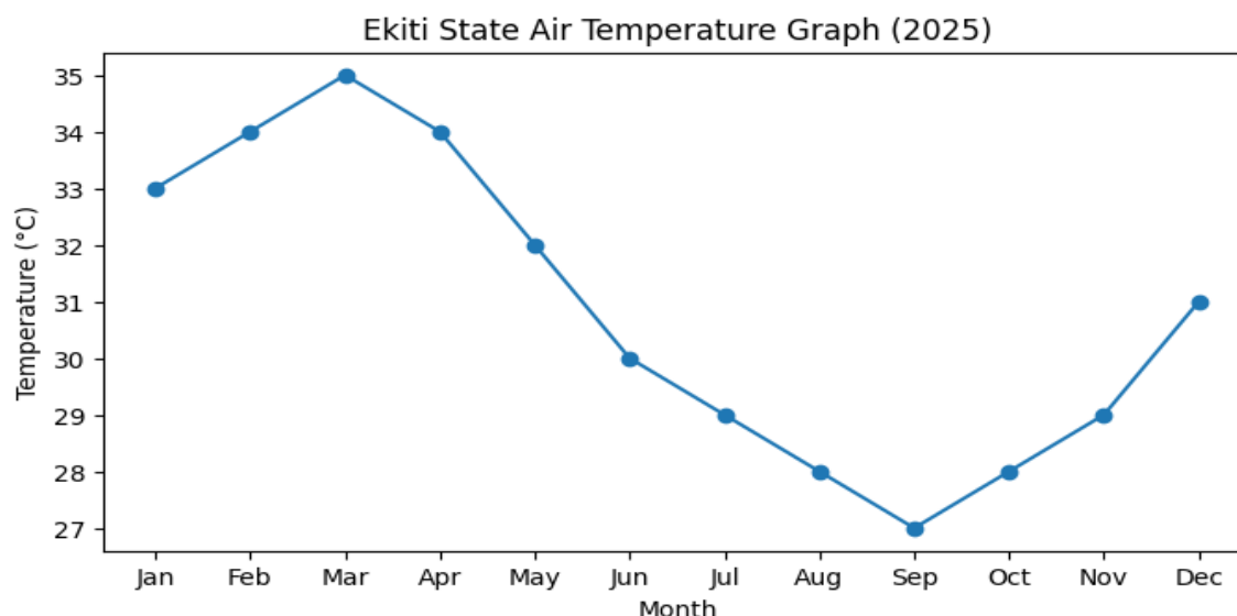
Figure 4.1: Monthly Temperature Distribution in the Proposed Area (Source: NIMET, 2025)
