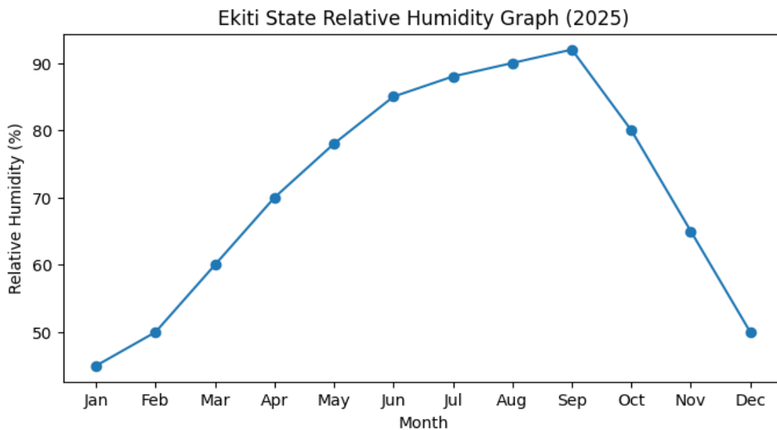
Figure 4.3: Relative Humidity in the Proposed Project Area (Source: NIMET, 2025)
