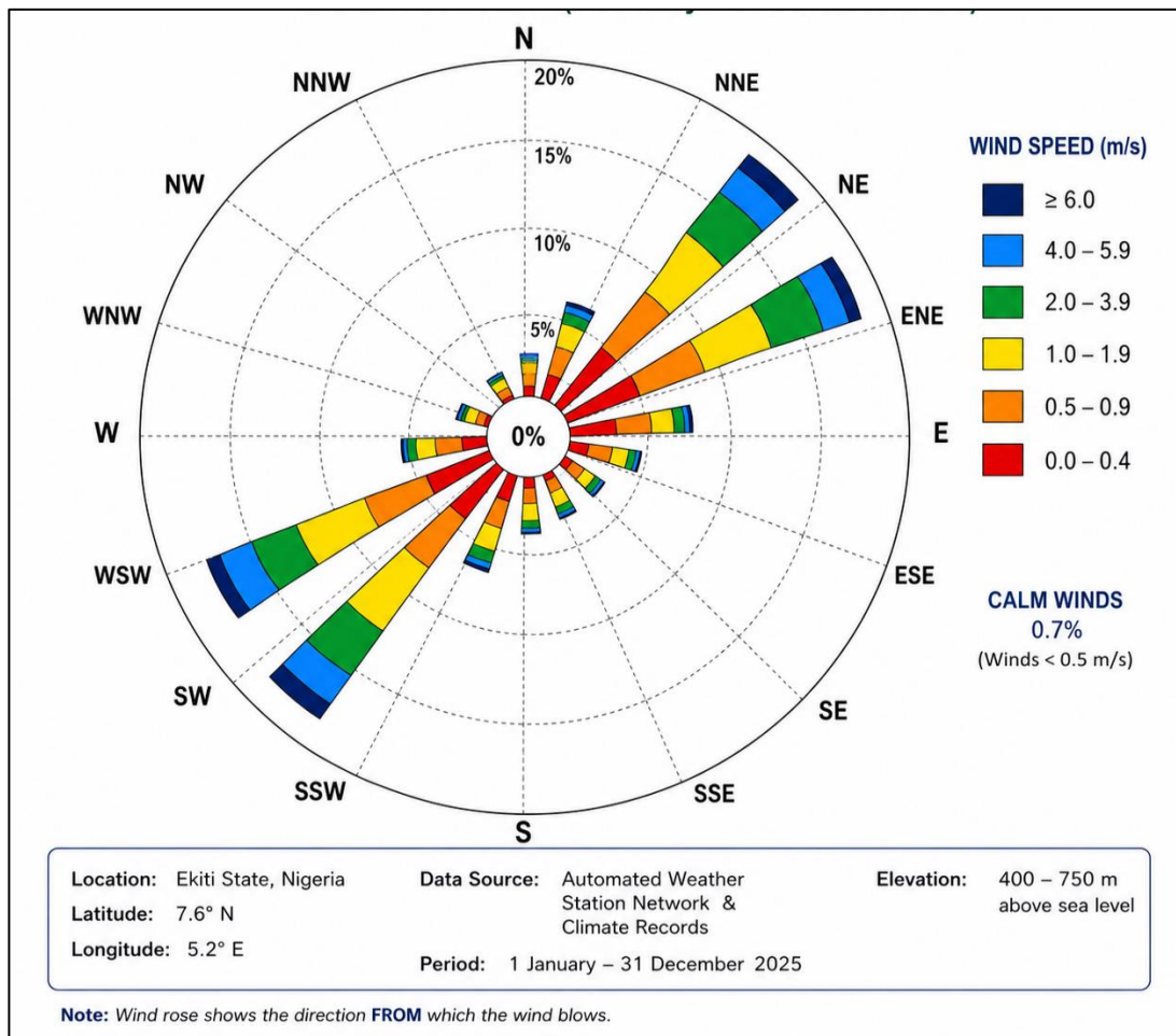
Figure 4.4: Surface Windrose of the Proposed Project Area (NIMET, 2025)
